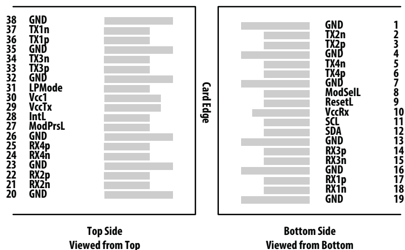
Figure 5: Host Board Pattern for QSFP28 Transceiver
