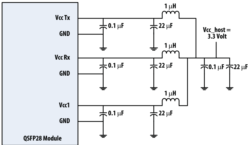
Figure 7: Recommended Power Supply Filter
