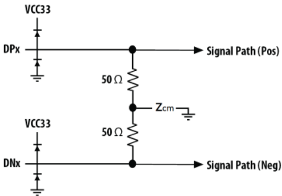
Figure 8: Transmitter Data Input Equivalent Circuit
