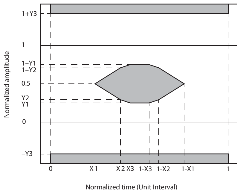
Figure 4: Transmitter Eye Mask Definitions
