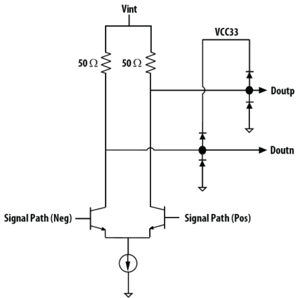
Figure 9: Receiver Data Output Equivalent Circuit
