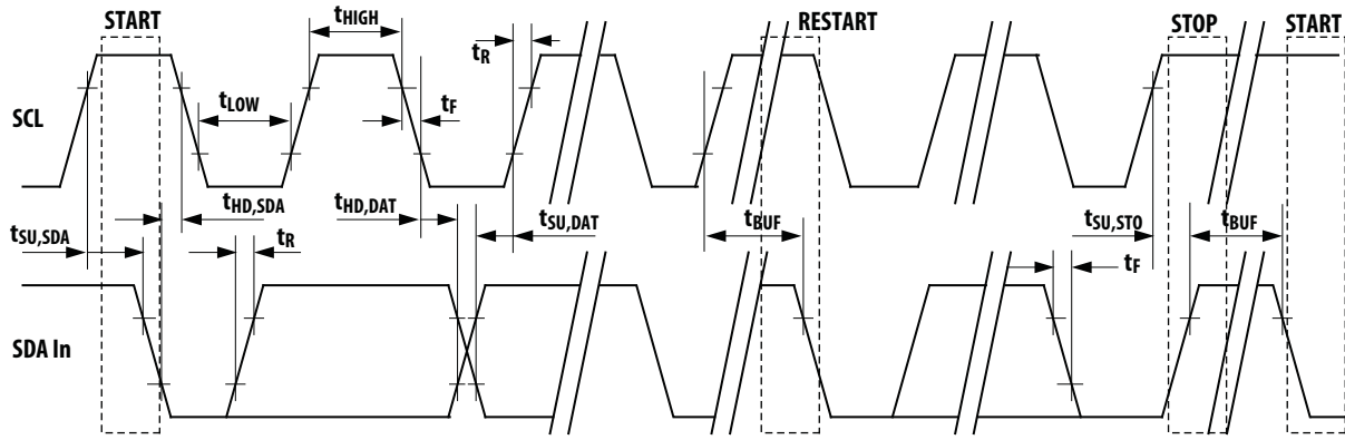
Figure 10: TWS Interface Bus Timing
