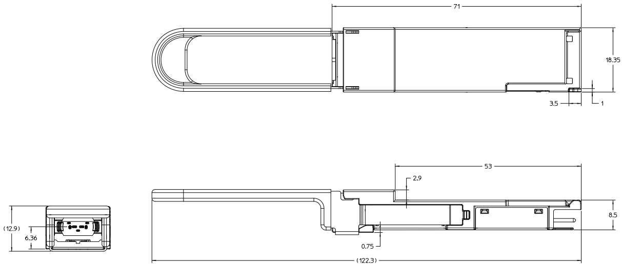
Figure 11: Mechanical Package Outline (All dimensions in mm)
