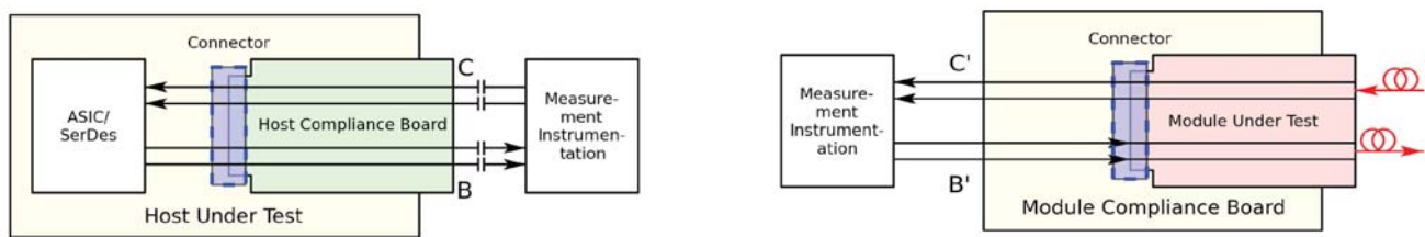
Figure 3. PC-PI-6P Compliance Points
